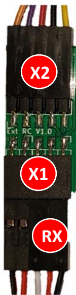
Top View – External Power Supply Connected
