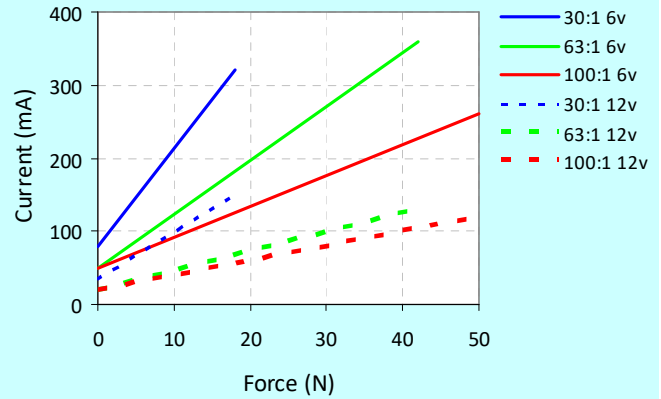
Current Curves
